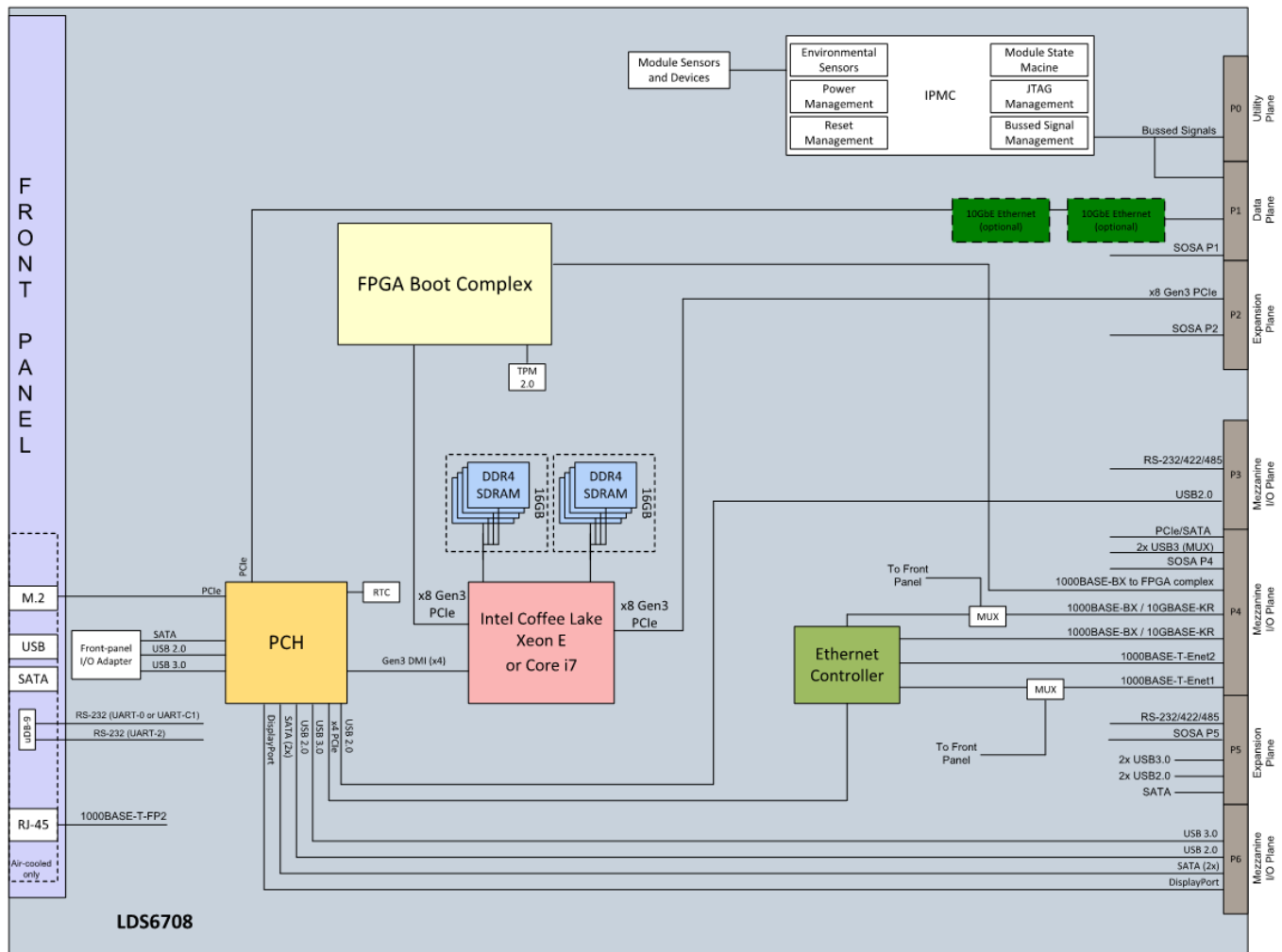
LDS6708 functional block diagram
